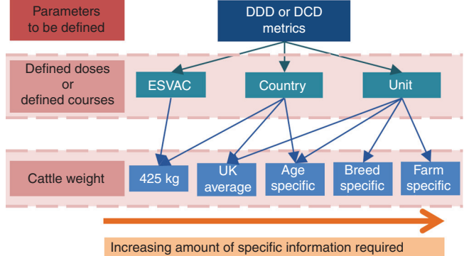
FIG 1: Flow chart explaining the different options for defined daily dose (DDD) and defined course dose (DCD) metrics. These metrics can (and have) been defined at European Surveillance of Veterinary Consumption (ESVAC) group, country or unit level, requiring doses or courses to be defined or known specifically for that level. These metrics also require cattle weights, and the ESVAC, country or unit level may define weight in different ways. The amount of specific information required increases from left to right in the figure as metrics become more representative of the actual situation on farms, with a trade-off of increasingly granular information necessary to calculate the metrics.
