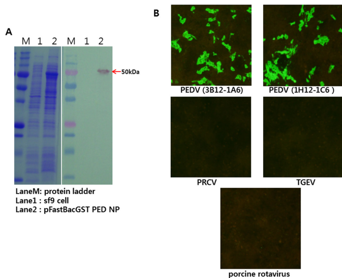
FIG 1: SDS-PAGE and western blot analysis for the expressed N protein of PEDV (A). Lane M: protein ladder; lane 1: Sf-9 cell; lane 2: expressed N protein of PEDV. SDS-PAGE gel viewed after Coomassie blue staining and western blot showing the protein detected using polyclonal anti-PEDV. The specificity of PEDV mAb by indirect immunofluorescence assay (B). Vero cells infected by PEDV and stained with PEDV mAbs (3B12-1A6 or 1H12-1C6) show typical cytoplasmic fluorescence, while cells infected by other porcine viruses and stained with PEDV mAbs (3B12-1A6 or 1H12-1C6) did not show the fluorescence. PEDV, porcine epidemic diarrhoea virus; PRCV, porcine respiratory coronavirus; Sf-9, Spodoptera frugiperda ; TGEV, transmissible gastroenteritis virus.
